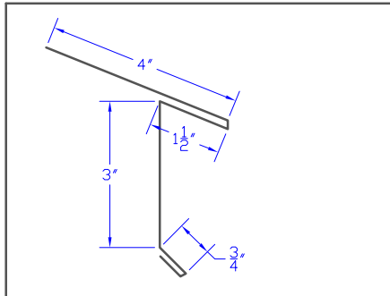
204 ST70 Extended Drip Edge 9.875'
