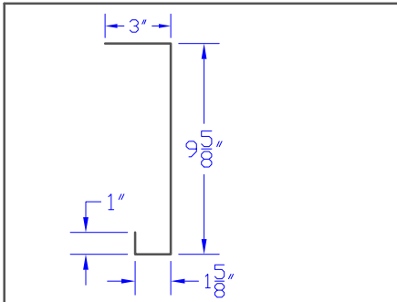
203 ST49 Fascia Board Cover 15.25'
