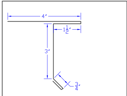
205 ST71 Extended Drip Edge 9.875'
