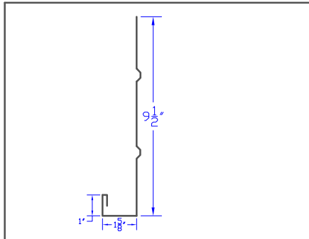
39 FR10 - 9 1/2' Ribbed Facia 12.625'
