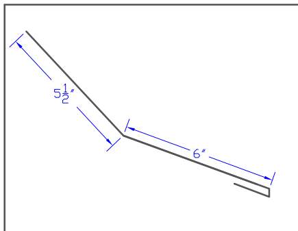
42 RT2 - Roof Transition 2 12'
