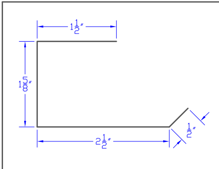
55 Dekk-Tile 2 C Channel 6.125"
