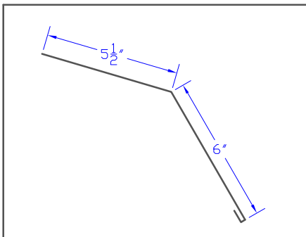
41 RT1 - Roof Transition 1 12'
